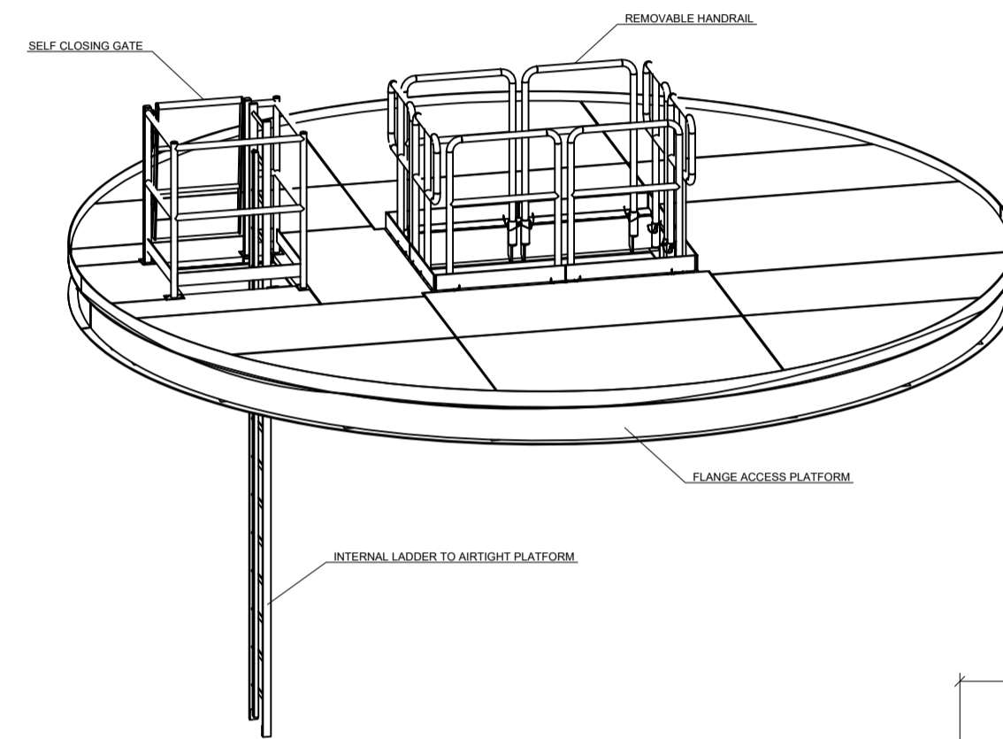
FLANGE ACCESS PLATFORM 3D VIEW: 1:50
