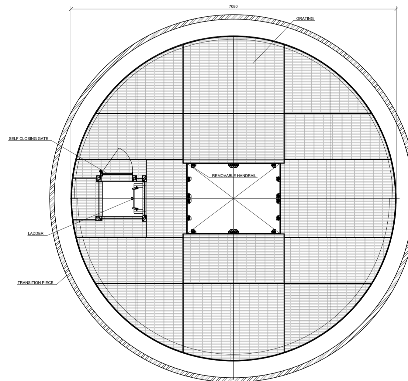
FLANGE ACCESS PLATFORM PLAN VIEW: 1:50
